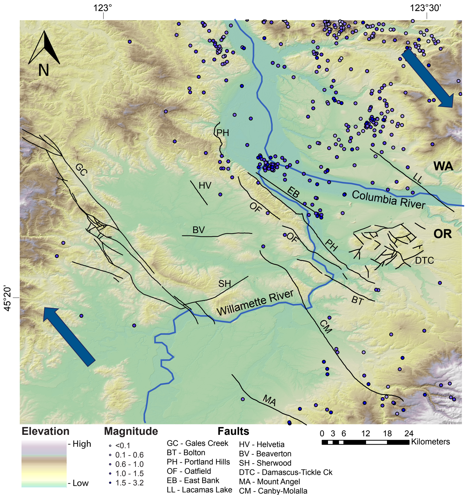
Map of Portland and Tualatin Basins showing microseismicity (data from Pacific Northwest Seismic Network) and the 12 faults included in this study. Locations for all faults except Gales Creek are from Quaternary Fold and Fault Database. Gales Creek Fault is mapped by Wells and others in press (2018). Blue arrows show relative sense of motion on the faults. Downtown Portland is denoted by a red star. Area of Figure 2 (GCF) is shown by the red box.
