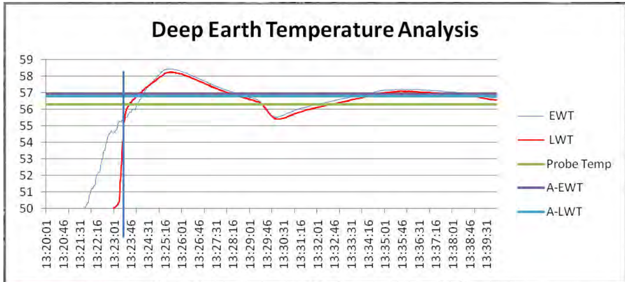
Figure 4 - Average Deep Earth Ground Temperature Analysis
