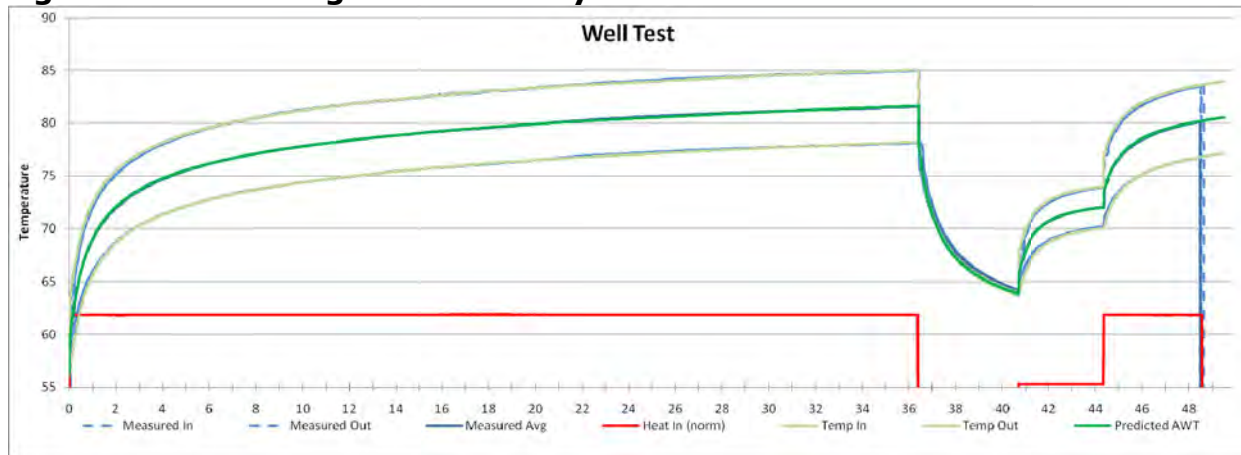
Figure 1 – A-TRT Digital Twin Analysis Results
