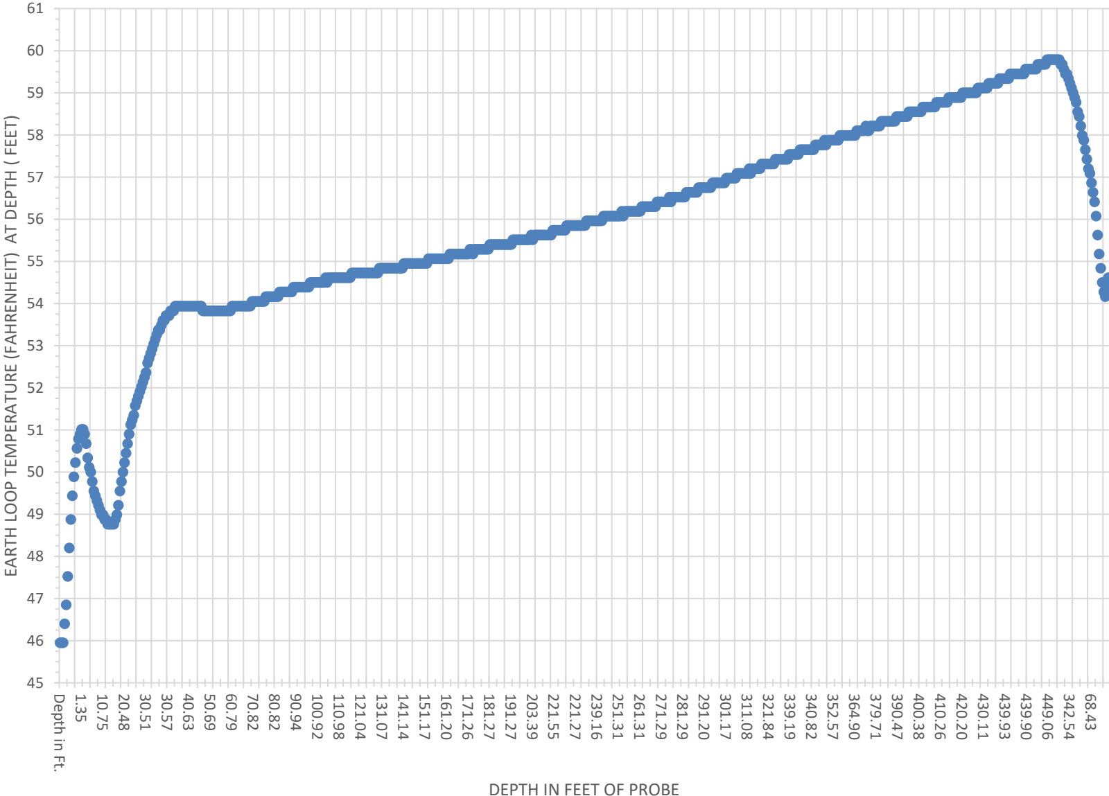
Probe Test of Deep Earth Temperature (°F)
