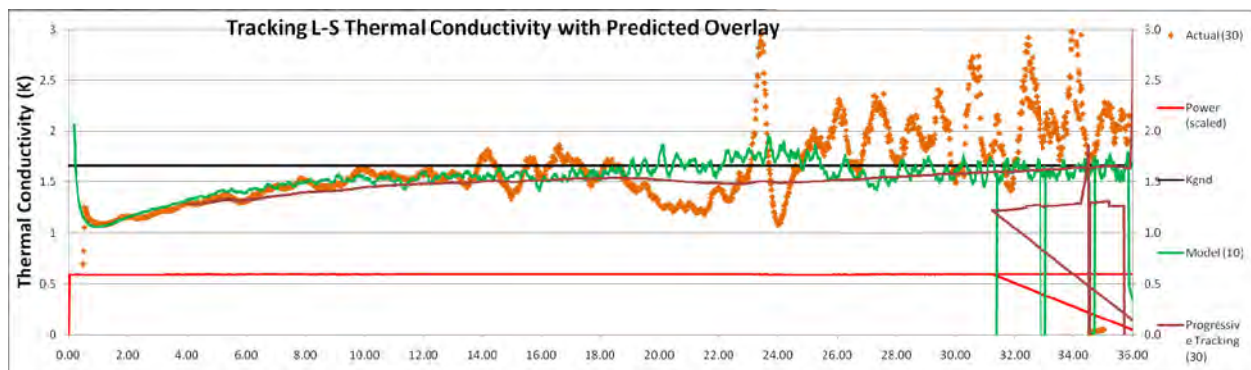
Figure 2 - A-TRT Tracking Analysis Results
