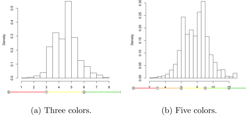
Figure 39: Histograms of the combined risk metric using a sum with 3- and 5-color schemes for geology only. Density is proportional to the frequency or count in the bins, but the values have been rescaled so the total area of the histogram is 1.
