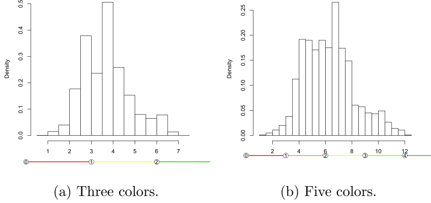
Figure 48: Histograms of the combined risk metric using a sum with 3- and 5-color schemes for all risk factors except reservoirs. Density is proportional to the frequency or count in the bins, but the values have been rescaled so the total area of the histogram is 1.
