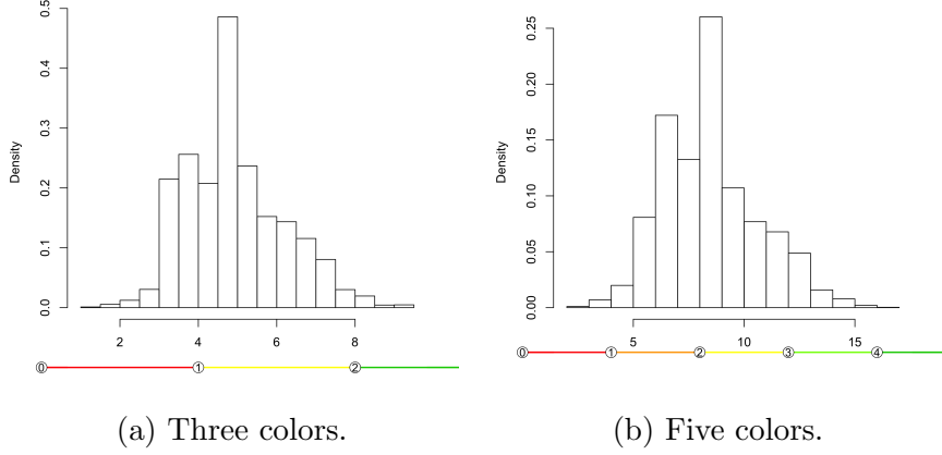
Figure 30: Histograms of the combined risk metric using a sum with 3- and 5-color schemes. Density is proportional to the frequency or count in the bins, but the values have been rescaled so the total area of the histogram is 1.
