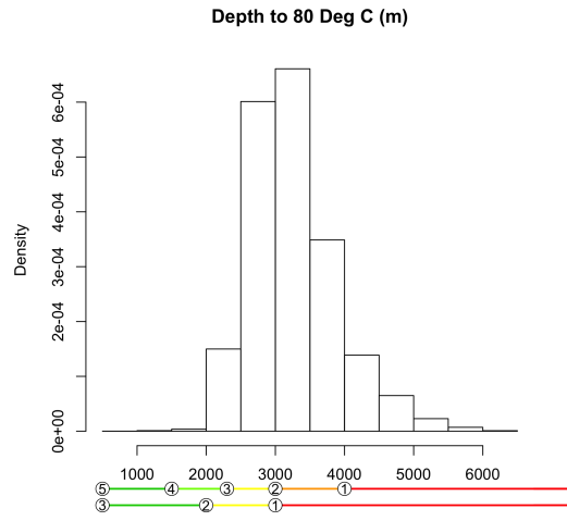
Figure 1: Histogram of the thermal risk factor with the 3- and 5-color thresholds noted. Points beyond the minimum and maximum of the scale are assigned the minimum and maximum of the scale, respectively (e.g. 0, and 3 or 5). Density is proportional to the frequency or count in the bins, but the values have been rescaled so the total area of the histogram is 1.
