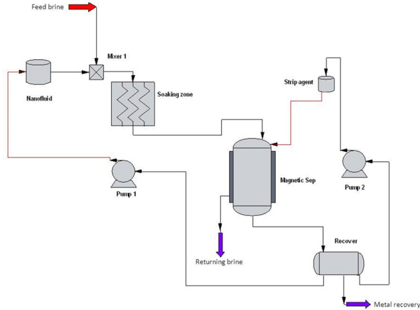
Figure 3. Rare earth metal extracting process using magnetic nanofluids
