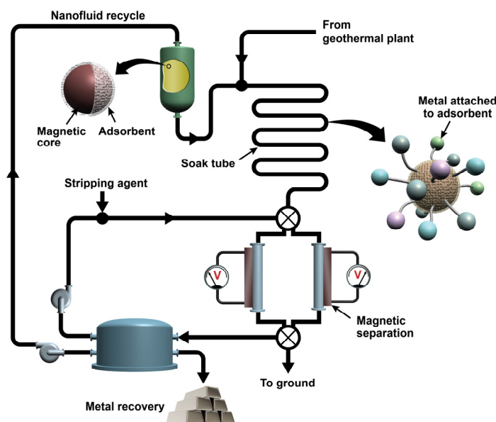
Figure 1. Conceptual drawing of magnetic partitioning nanofluid extraction system
