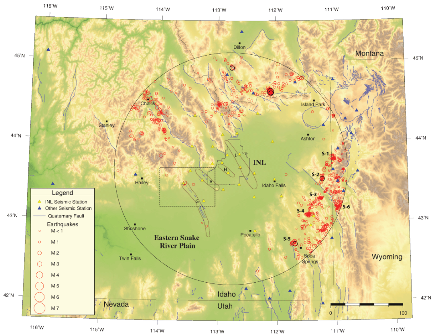
Figure 6. Map of epicenters of earthquakes within the 161-km radius around the INL from January 1, 2011 to December 31, 2011. Dashed box shows the region for Figure 7. Earthquake swarms are identified as S-#. Earthquakes of magnitude \geq 3.0 are outlined in dark blue. See Figure 1 for abbreviations.
